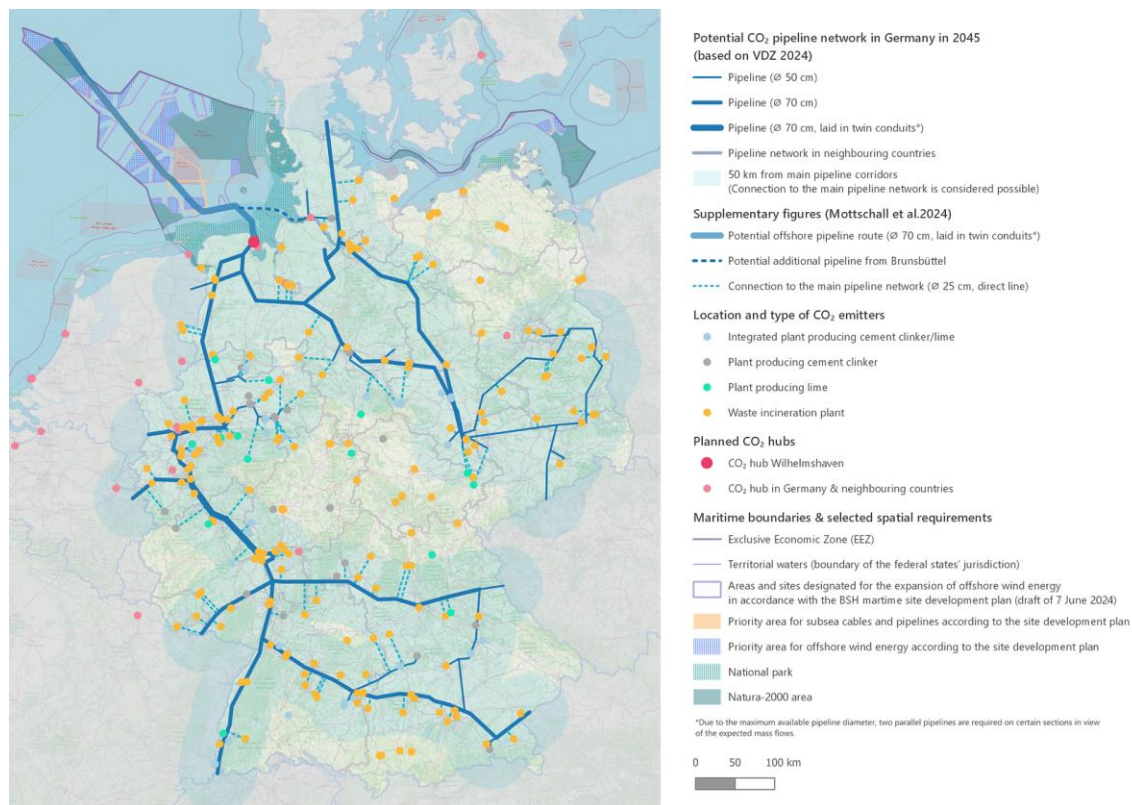
Figure 11-8: Structures of a prospective CO 2 network in Germany in 2045
