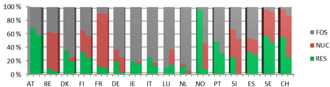
Figure 3. Generation (left) and residual (right) mixes of 2011 of selected European countries based on [38].
