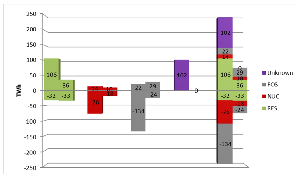
Figure 5. Total quantified implicit disclosure errors per energy source before 2010 (left-hand columns) and after 2012 (right-hand columns) RE-DISS.
