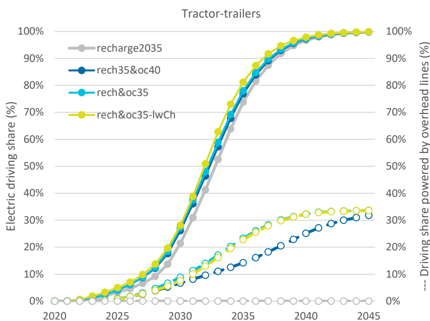
Figure 5-16: Electric driving share in the "BEV+OC-BEV" scenarios
