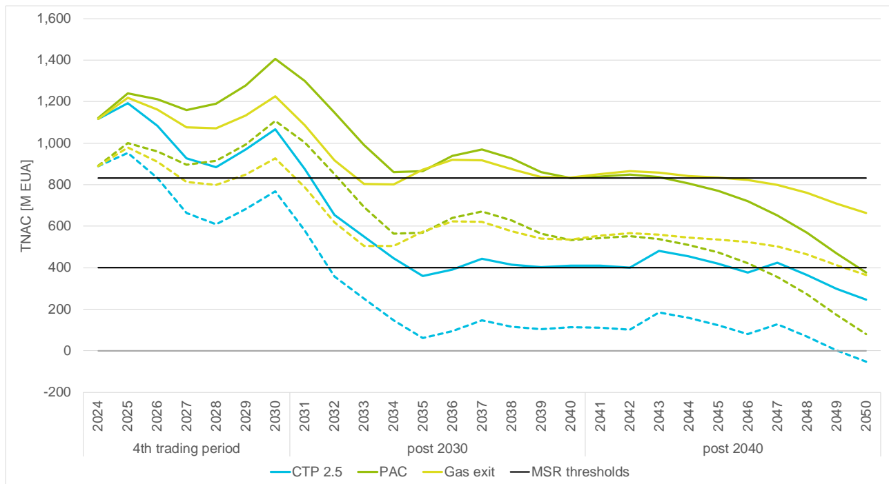
Figure 4-4: ETS 1: TNAC and TNAC_{VM} under an LRF of 2.2% from 2035 and 1.1% from 2040 onwards
